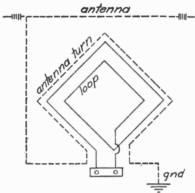
Fig. 1. By Combining Loop and Short Antenna, One Way Only is Picked Up.
