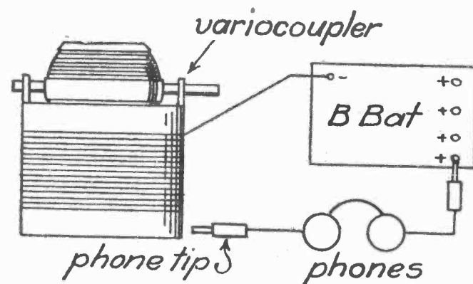
Fig. 2. How to Test an Instrument for Leakage.
