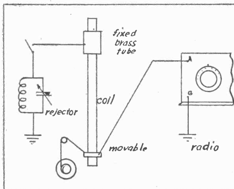
Fig. 2. The Sliding Coil in the Tube Short Circuits the Disturbance.
