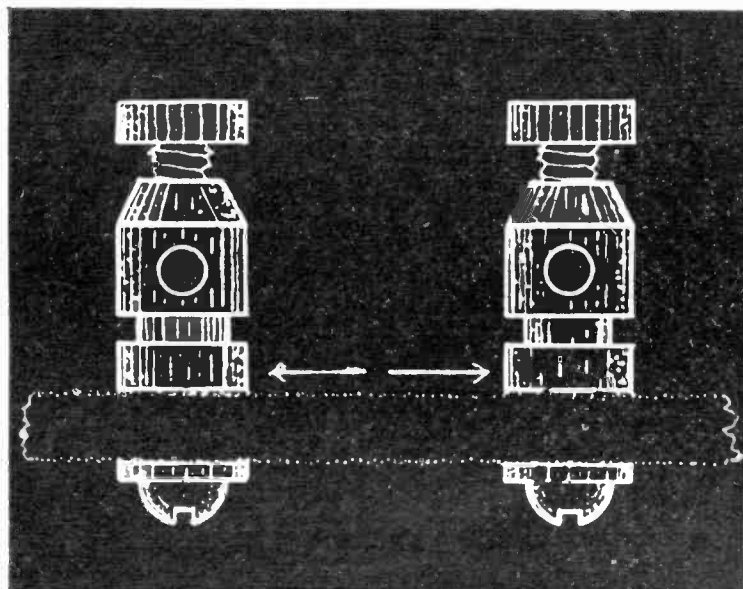
Fig. 1. The Arrows Show How High Frequency Alternating Currents Leak.
