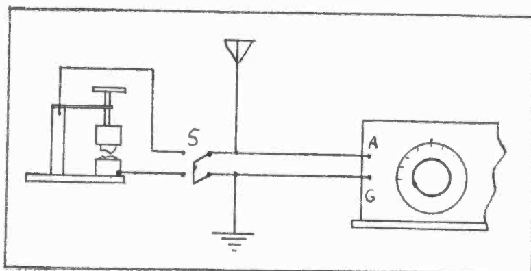
Fig. 1. This Crystal When Properly Adjusted Will Discourage Static.
