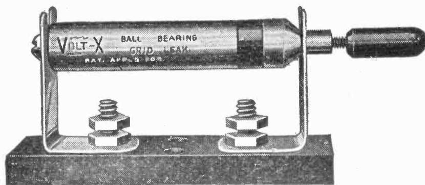
Volt-X Ball-Bearing Variable Grid Leak
