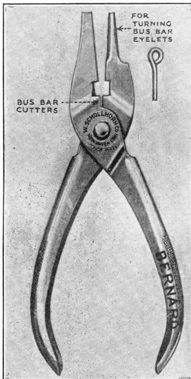
Fig. 2. Special Pliers That Will Make an Eye on the End of Bus Bar
