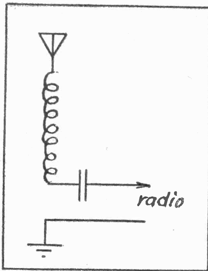
Fig. 3. This Acceptor Circuit Allows Only the Wanted Signal Through.
