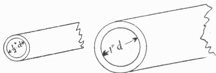
Fig. 1. Twice the Diameter Gives One-fourth the Resistance for Water or Electricity.
