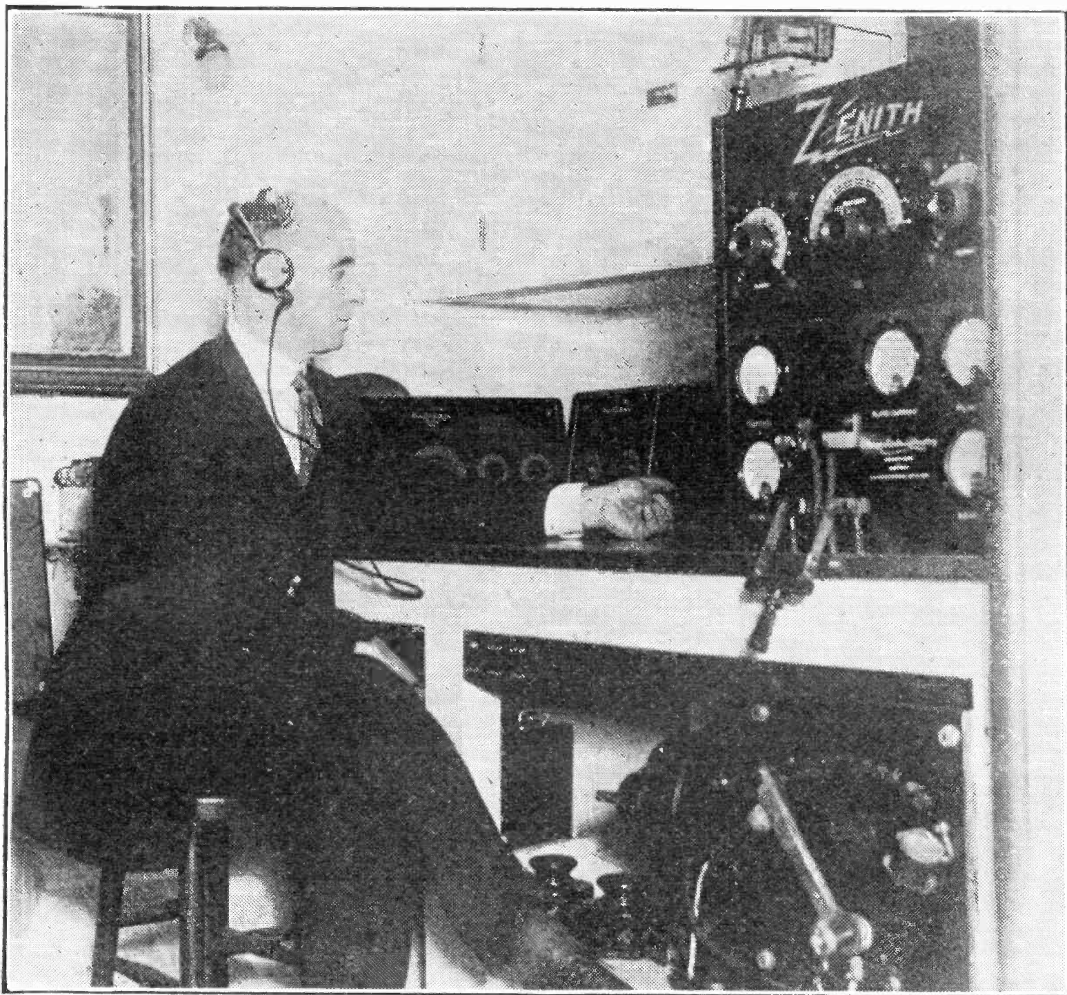
Fig. 2. MacMillan is Sending Out on 7,500 kc. (40 Meters) an Account of His Difficulties and Triumphs.
