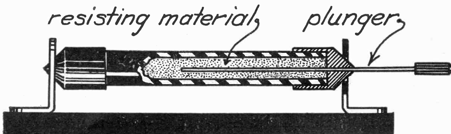
Fig. 6. The Basic Principle of Most Variable Leaks
