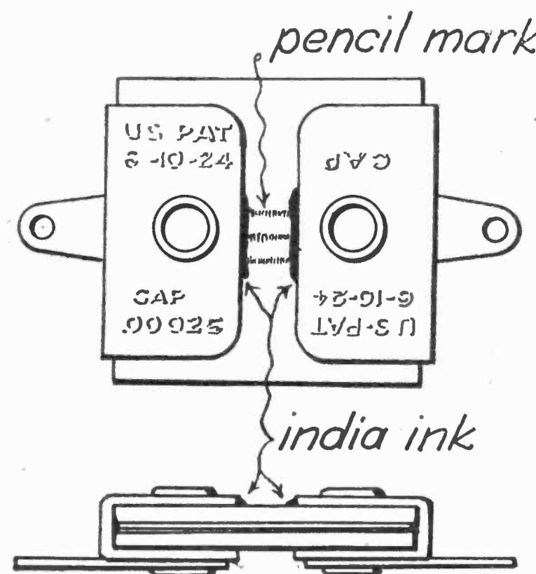
Fig. 9. The Home-made Leak. Don't Omit the India Ink
