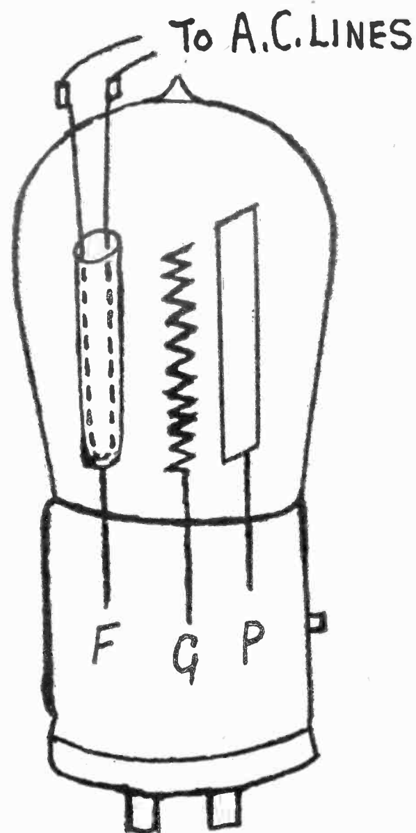
Fig. 2. Here is the Principle of the A. C. Vacuum Tubes
