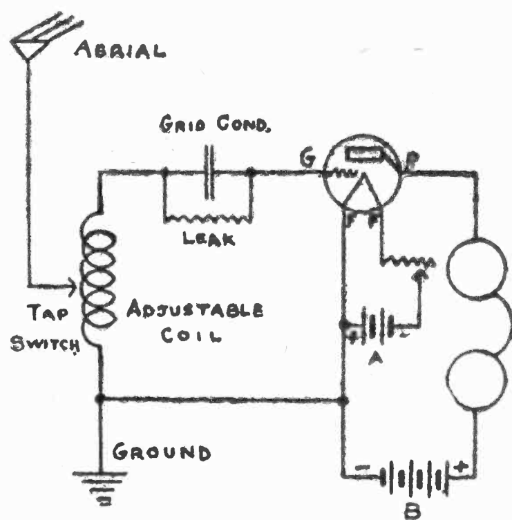
Fig. 1. This Hook-up Shows How Leak is Connected
